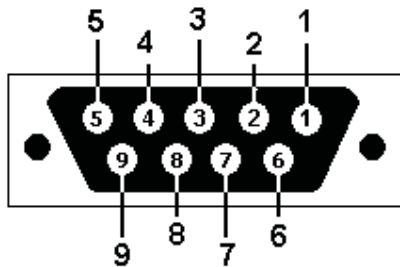
DB9 View Looking into Female Connector
