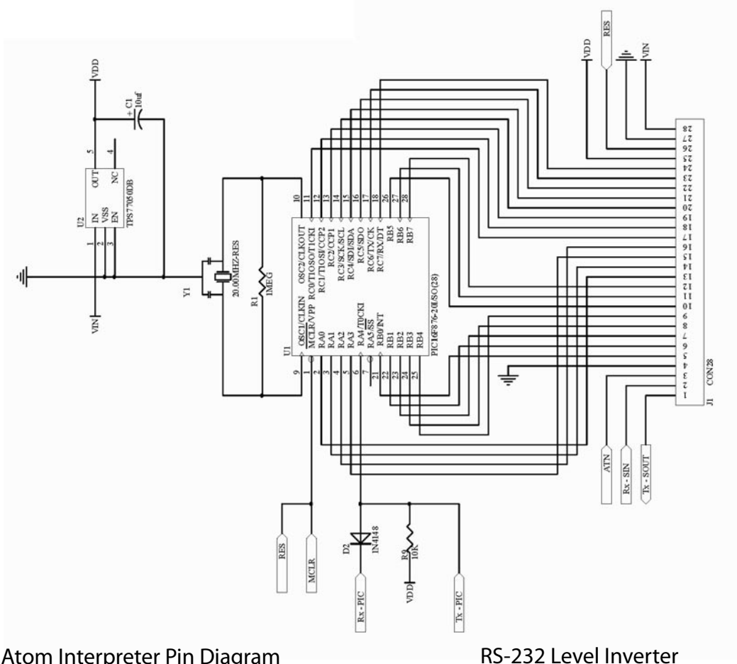
Atom Interpreter Pin Diagram
